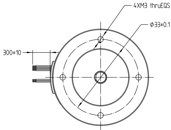
Mechanical View 1
