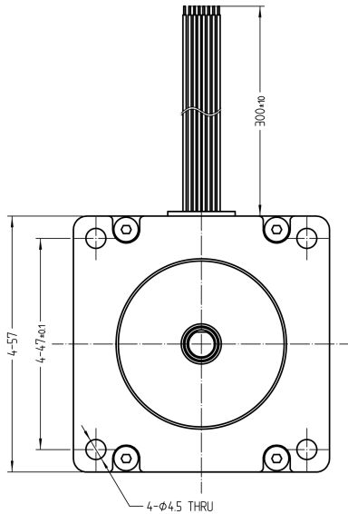
Mechanical View 1
