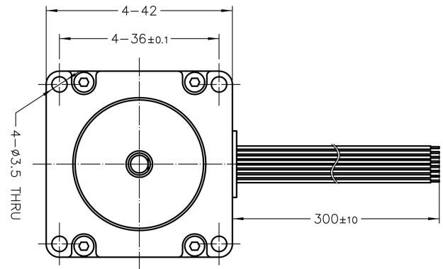
Mechanical View 2
