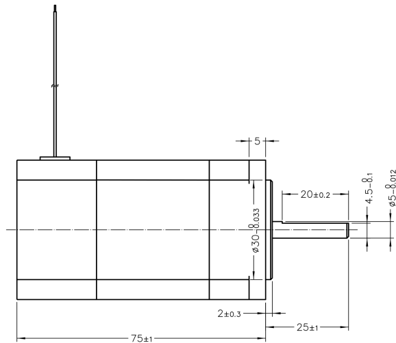
Mechanical View 1
