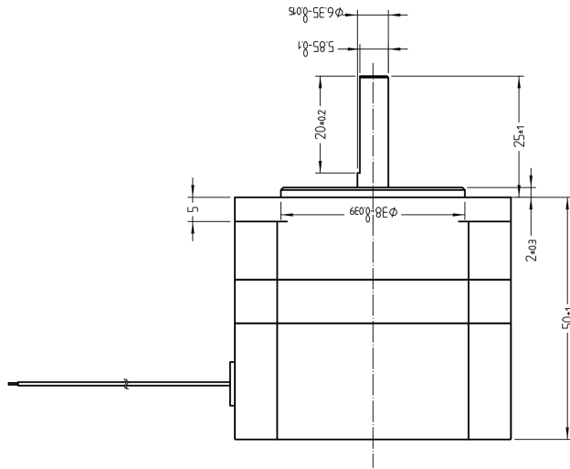
Mechanical View 1
