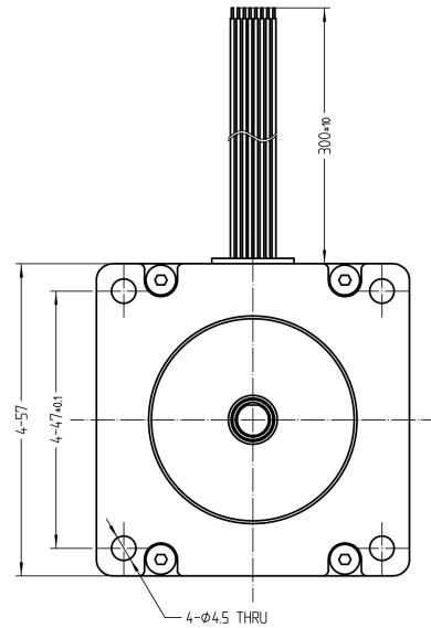
Mechanical View 2
