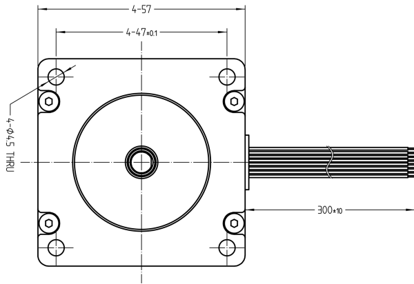
Mechanical View 1
