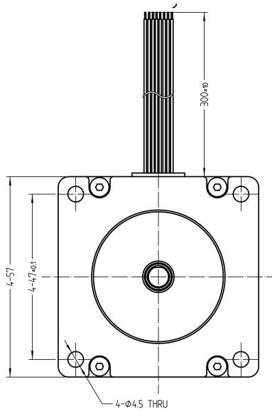
Mechanical View 1
