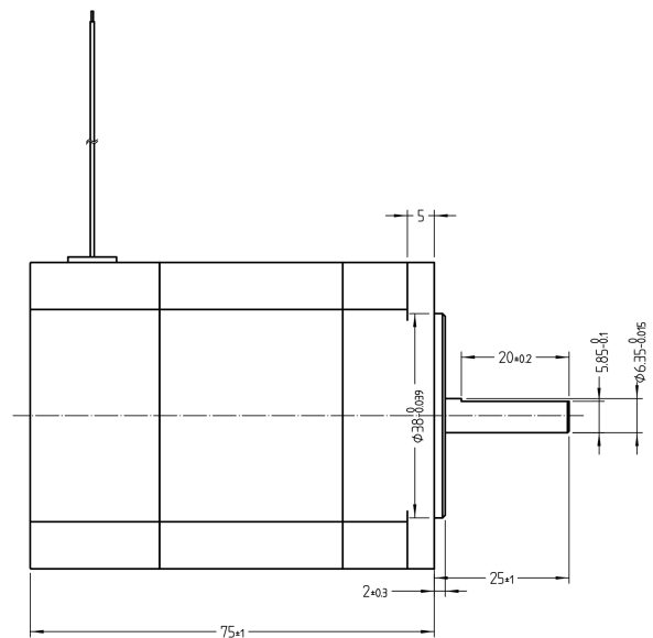
Mechanical View 2
