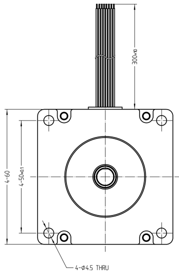
Mechanical View 1
