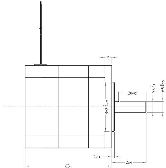
Mechanical View 2
