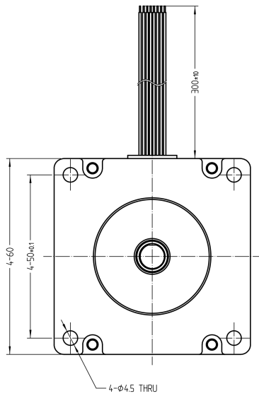
Mechanical View 1
