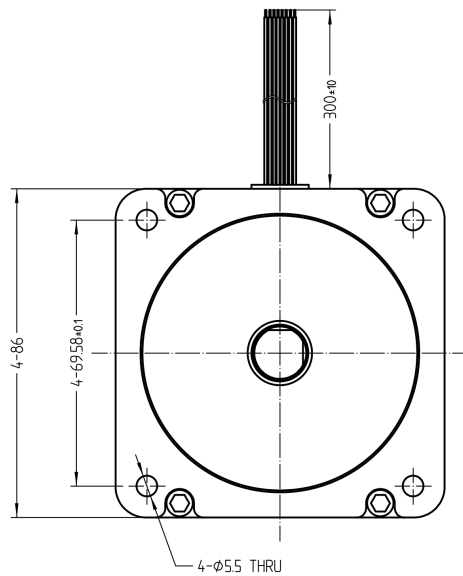
Mechanical View 1
