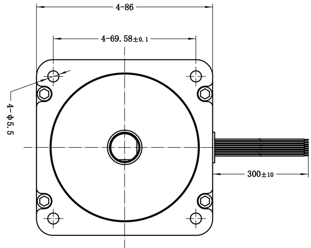
Mechanical View 2
