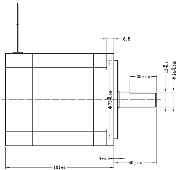
Mechanical View 1
