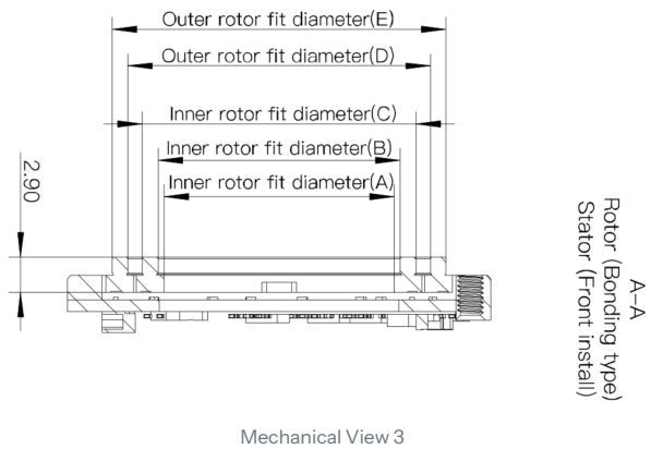
Mechanical View 3
