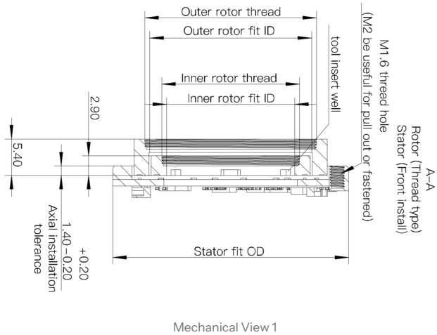
Mechanical View 1
