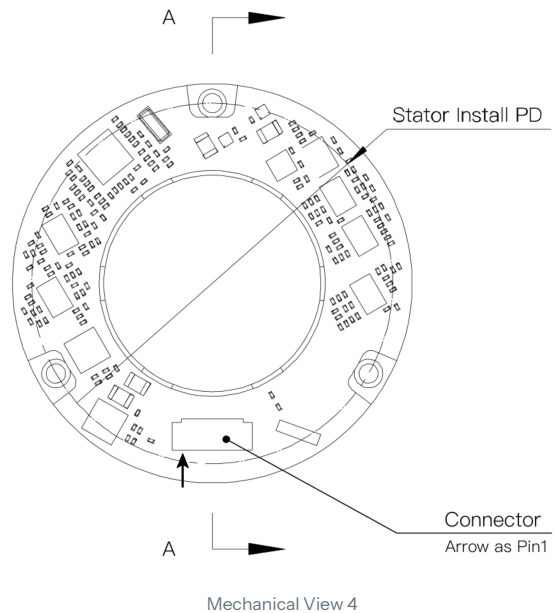
Mechanical View 4
