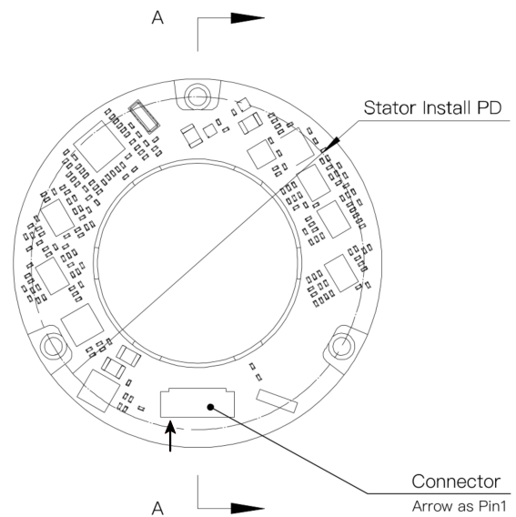
Mechanical View 4
