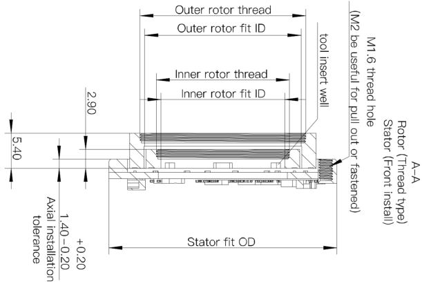
Mechanical View 1
