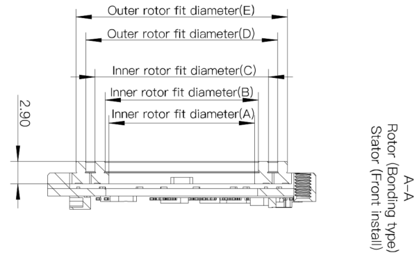
Mechanical View 2
