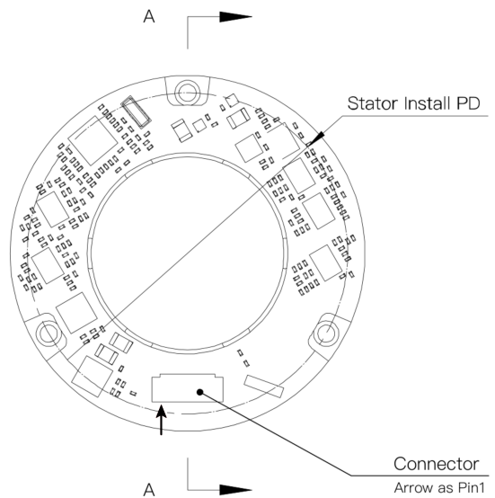
Mechanical View 4
