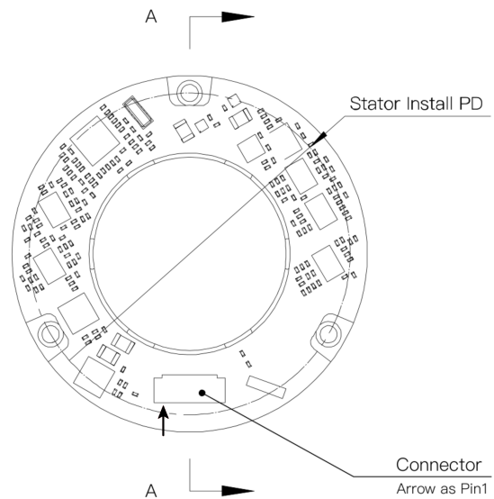
Mechanical View 4
