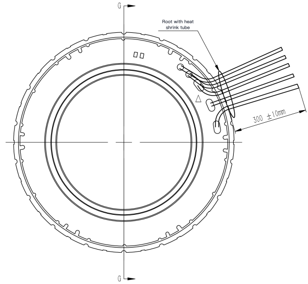
Mechanical View 2
