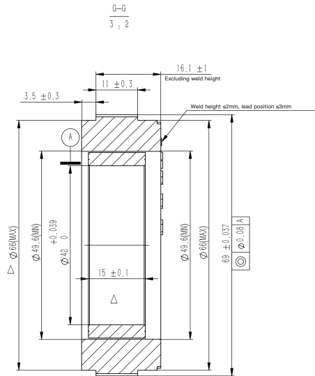
Mechanical View 1
