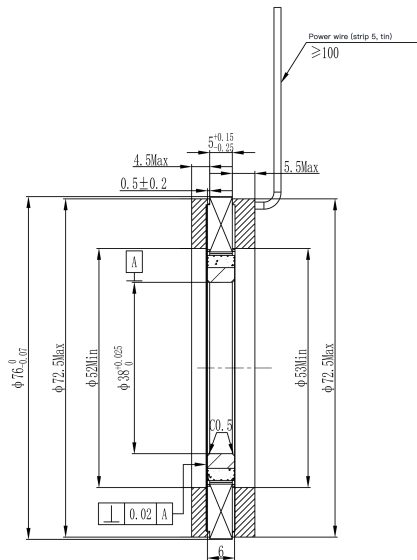
Mechanical View 1
