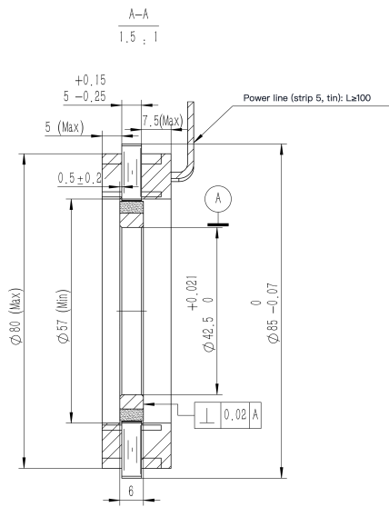
Mechanical View 3
