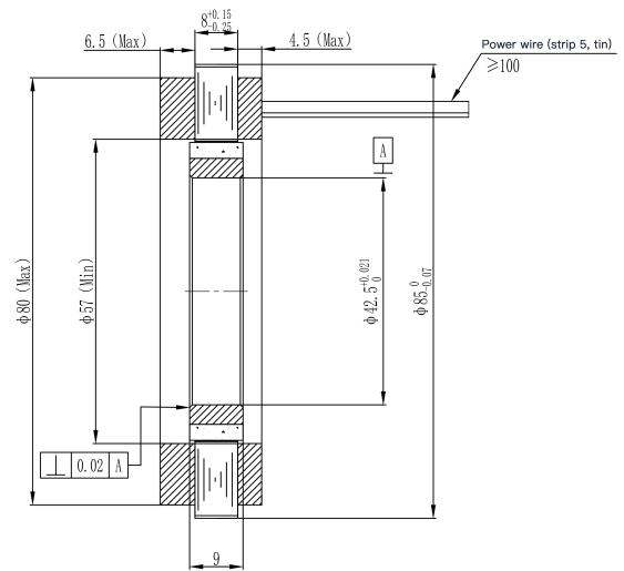
Mechanical View 2
