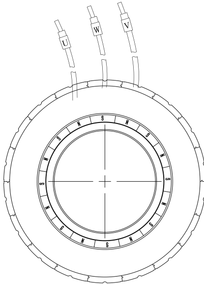
Mechanical View 1
