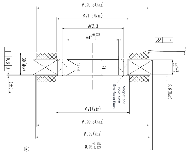
Mechanical View 3
