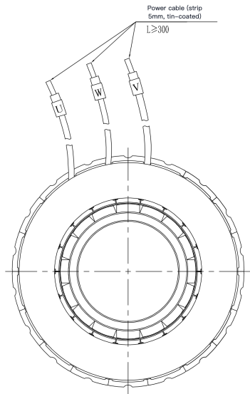
Mechanical View 2
