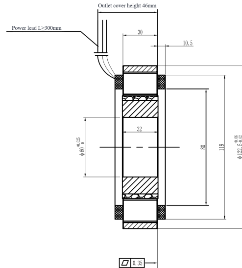
Mechanical View 3
