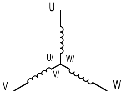
Wiring diagram (shaft end CCW)
