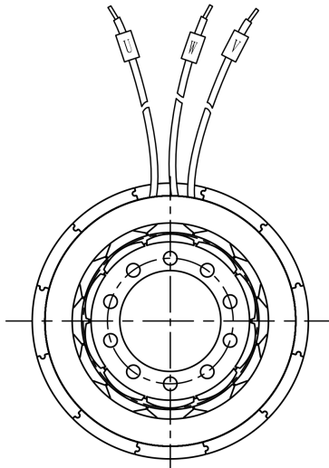
Mechanical View 2
