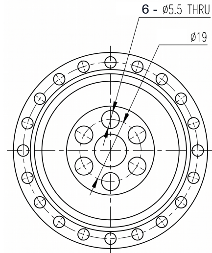
Mechanical View 2
