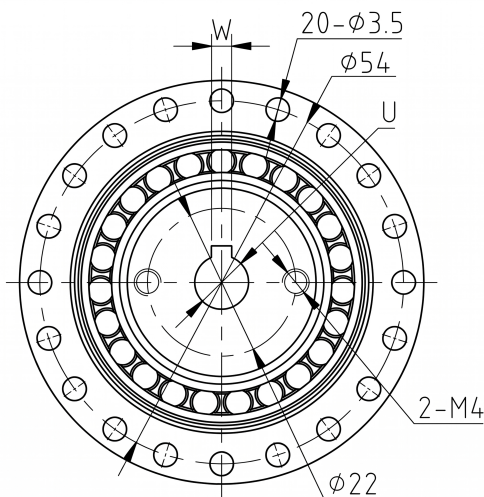
Mechanical View 3
