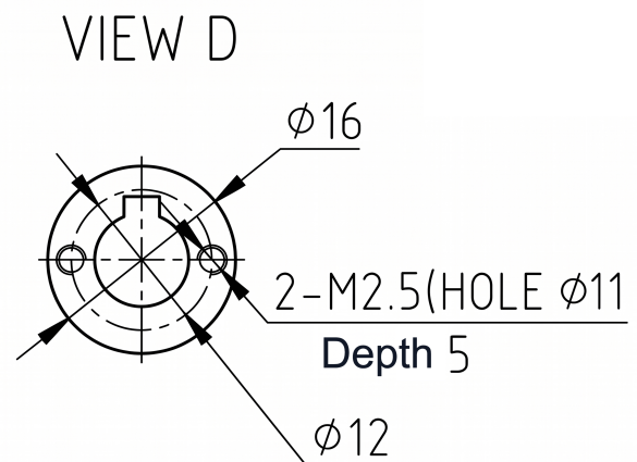
Mechanical View 4
