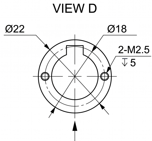
Mechanical View 4
