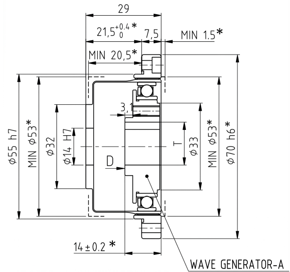
Mechanical View 2
