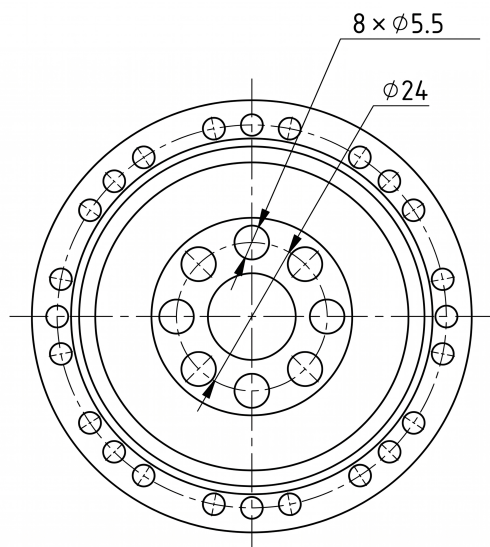
Mechanical View 3
