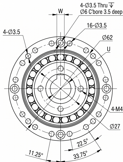
Mechanical View 1
