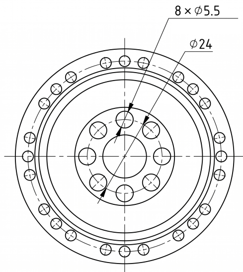
Mechanical View 3
