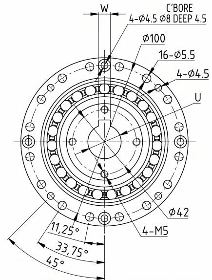
Mechanical View 2
