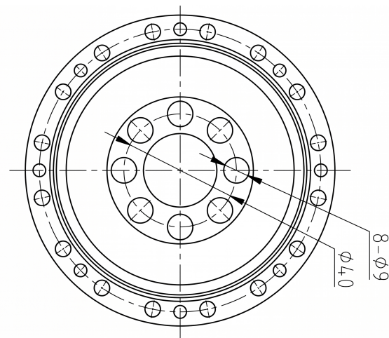
Mechanical View 3
