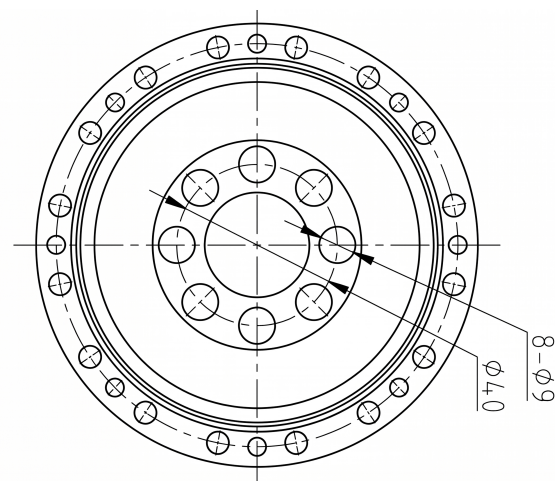
Mechanical View 3
