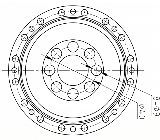
Mechanical View 3
