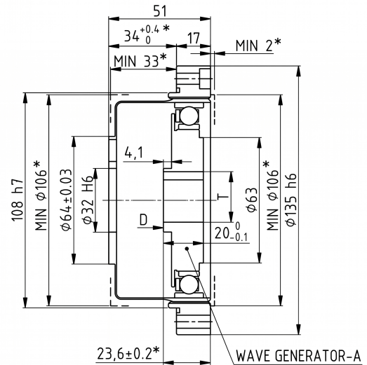
Mechanical View 2
