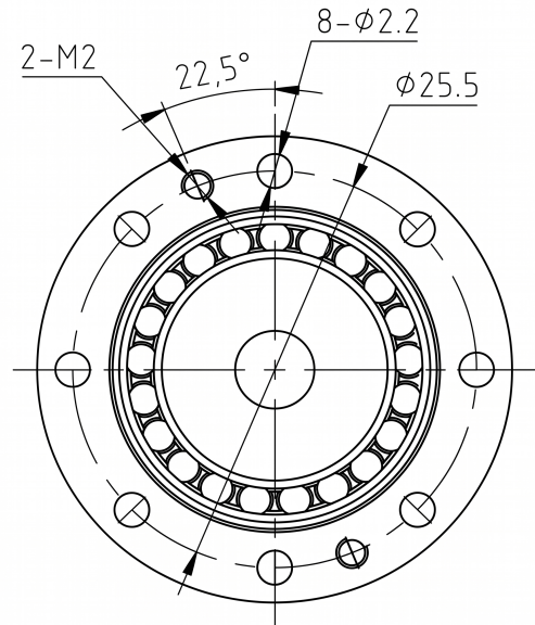
Mechanical View 2
