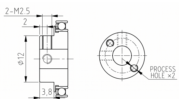
Mechanical View 4
