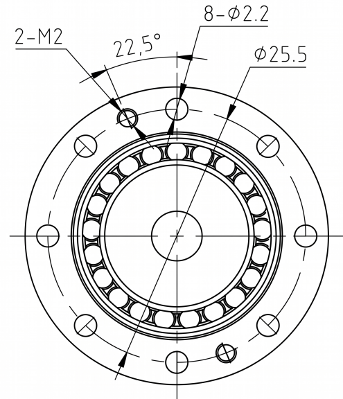
Mechanical View 2
