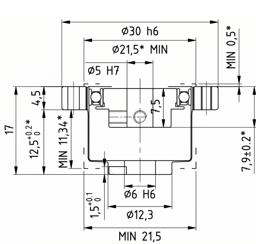
Mechanical View 1
