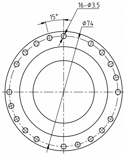
Mechanical View 1
