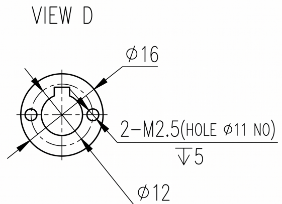
Mechanical View 4
