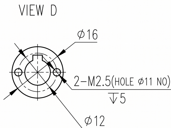
Mechanical View 4
