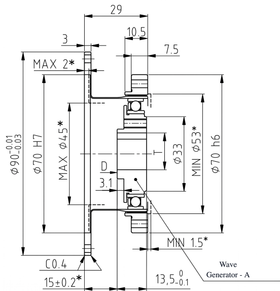
Mechanical View 1
