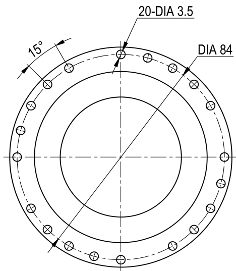
Mechanical View 3
