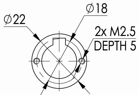
Mechanical View 4
