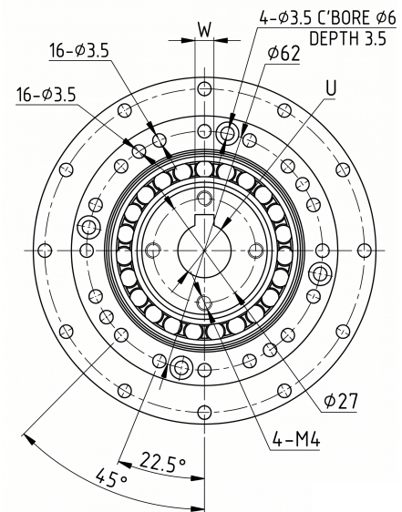
Mechanical View 2
