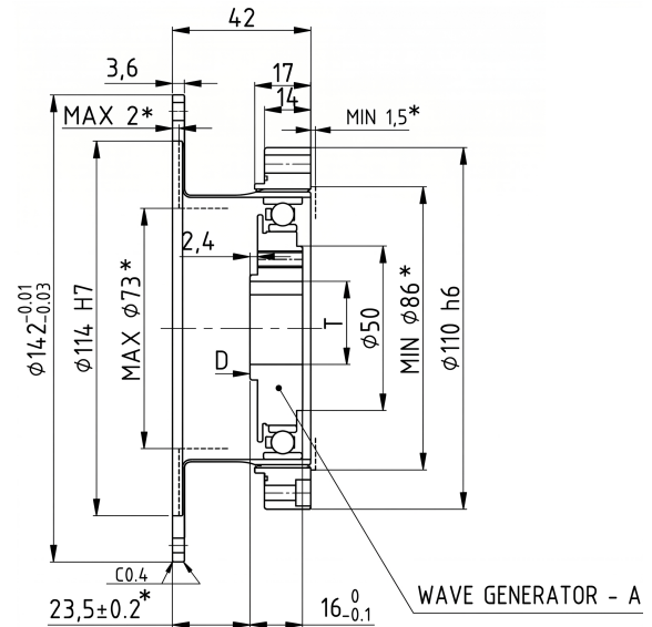
Mechanical View 2
