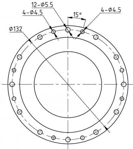
Mechanical View 1
