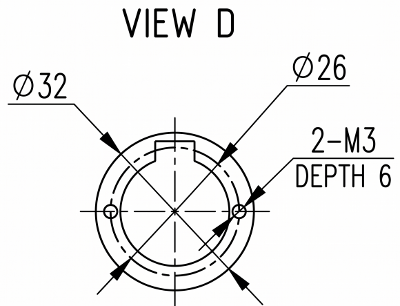
Mechanical View 4
