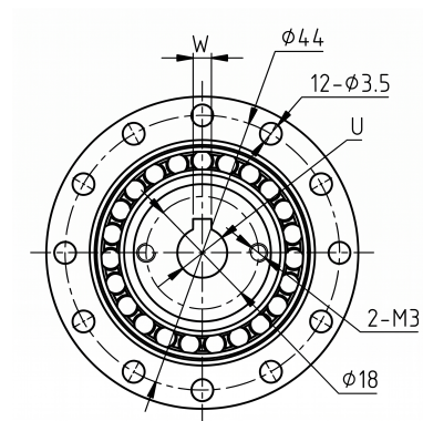
Mechanical View 2
