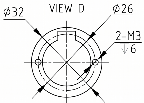
Mechanical View 2
