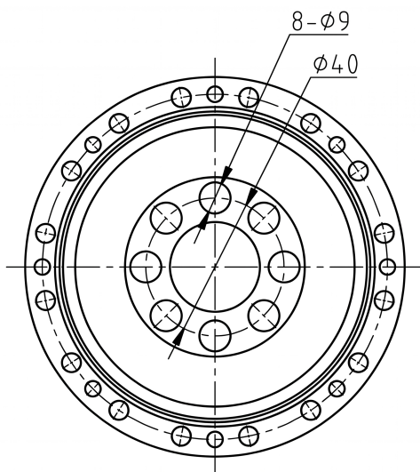
Mechanical View 3
