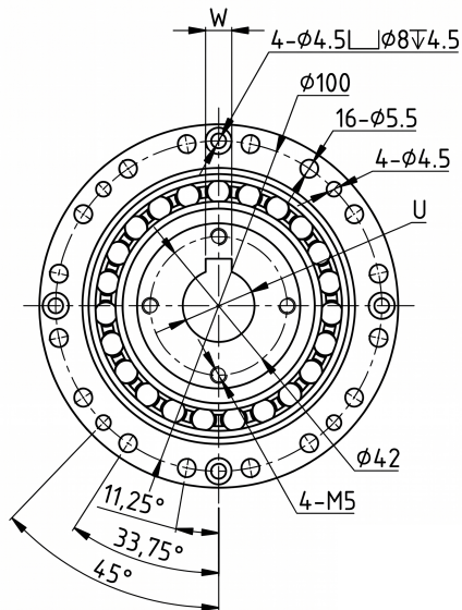
Mechanical View 1
