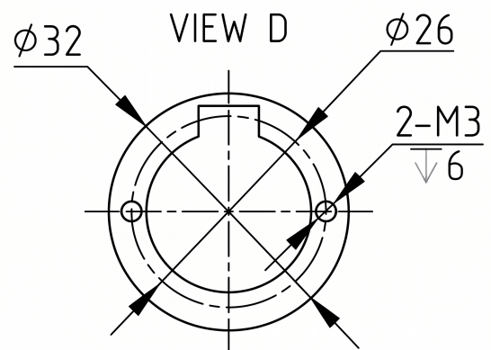
Mechanical View 2
