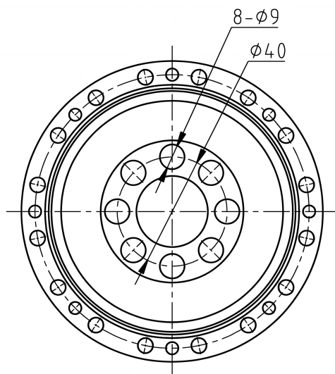
Mechanical View 3
