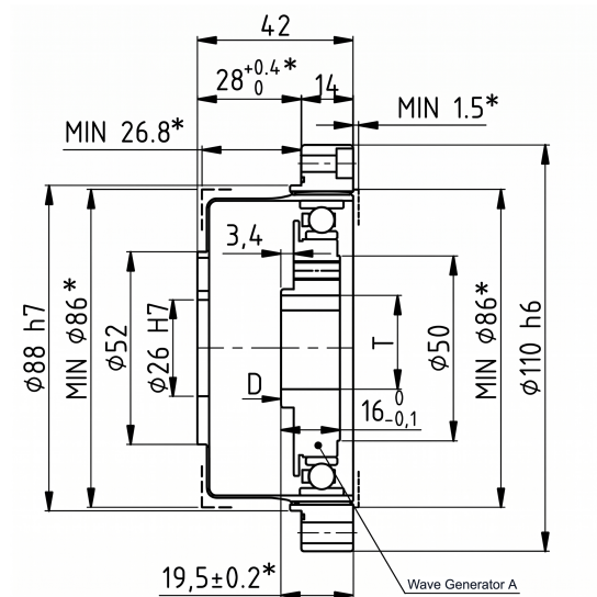
Mechanical View 2
