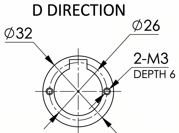
Mechanical View 4
