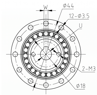
Mechanical View 3
