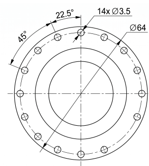
Mechanical View 2
