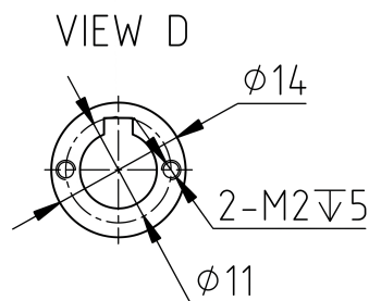
Mechanical View 5
