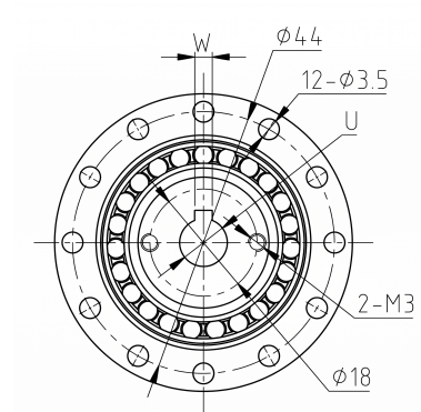
Mechanical View 3
