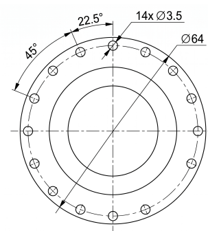
Mechanical View 2
