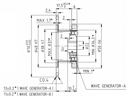
Mechanical View 1
