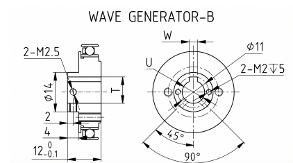
Mechanical View 4
