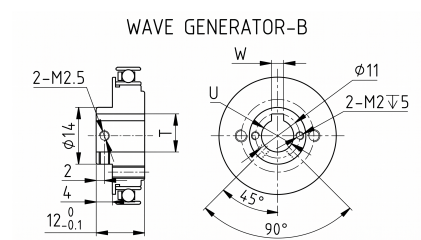
Mechanical View 4
