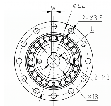
Mechanical View 3
