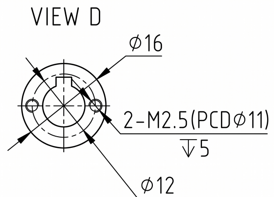
Mechanical View 4
