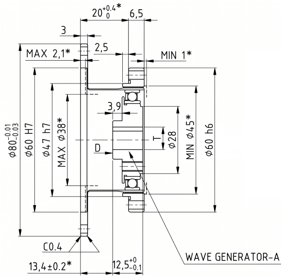
Mechanical View 1
