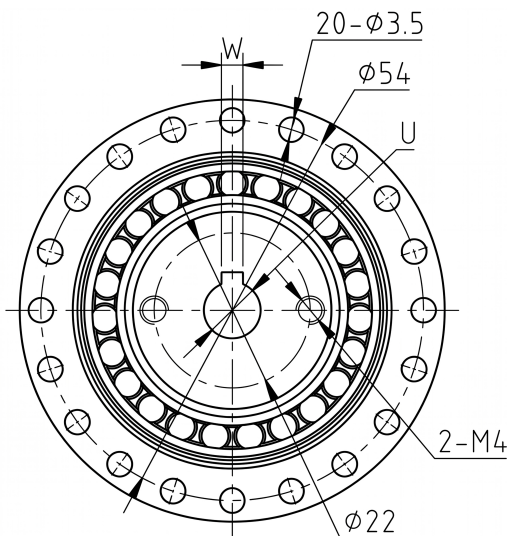
Mechanical View 3
