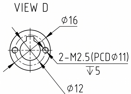
Mechanical View 4
