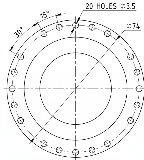
Mechanical View 2
