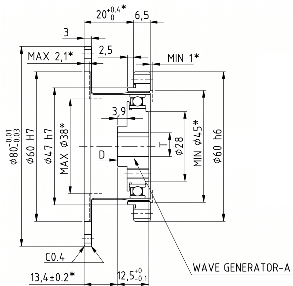
Mechanical View 1
