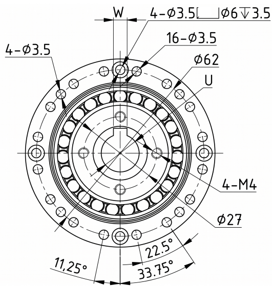
Mechanical View 3
