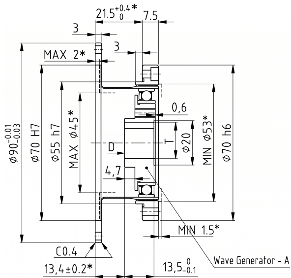
Mechanical View 1
