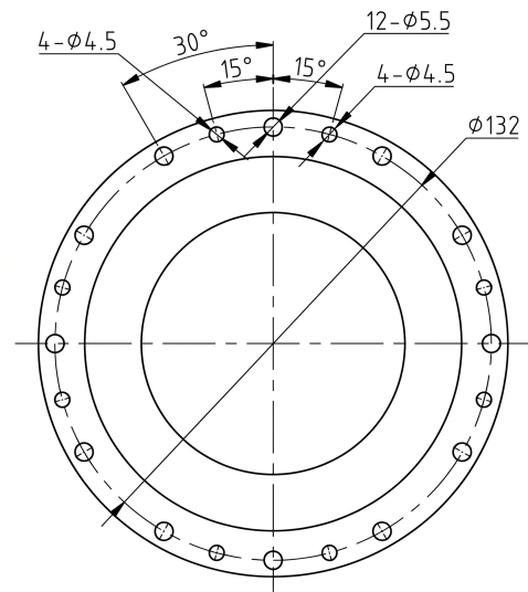
Mechanical View 2
