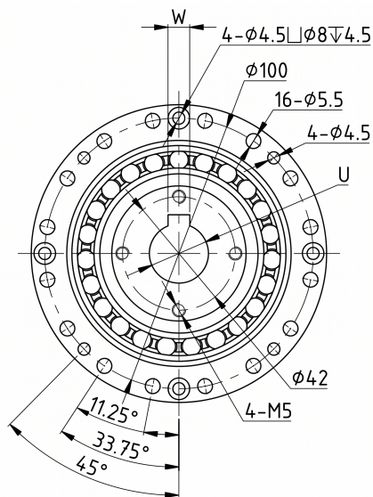
Mechanical View 3
