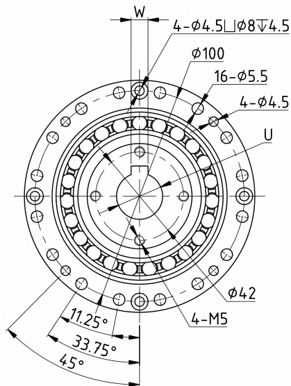
Mechanical View 3
