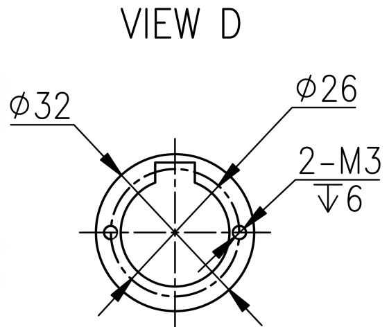
Mechanical View 4
